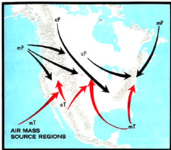
The oceans and the land are both important air-mass sources.
