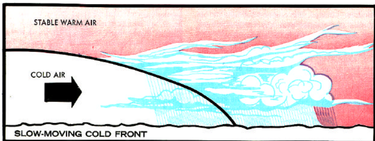
Clouds and precipitation cover a wide band and extend some distance behind slow-moving cold fronts. If the warm air is moist and stable, stratus-type clouds and steady rain occur. If the warm air is conditionally unstable, showers and thunderstorms are likely.
