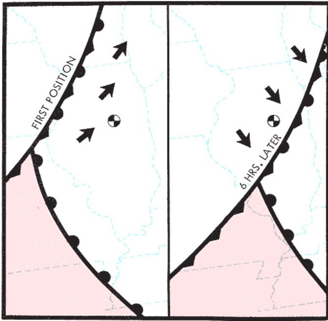
The wind shift accompanying the passage of an occluded front is usually 90° or more, generally from a southerly to a westerly or northwesterly direction.
