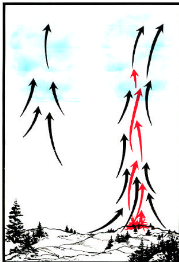
In the cumulus stage, the principal effect of a thunderstorm on a going fire is produced by the updraft. As a cumulus cloud drifts over a fire, the updraft into the cloud and the convection column over the fire reinforce each other. The updraft is strengthened, and spotting potential is increased.
