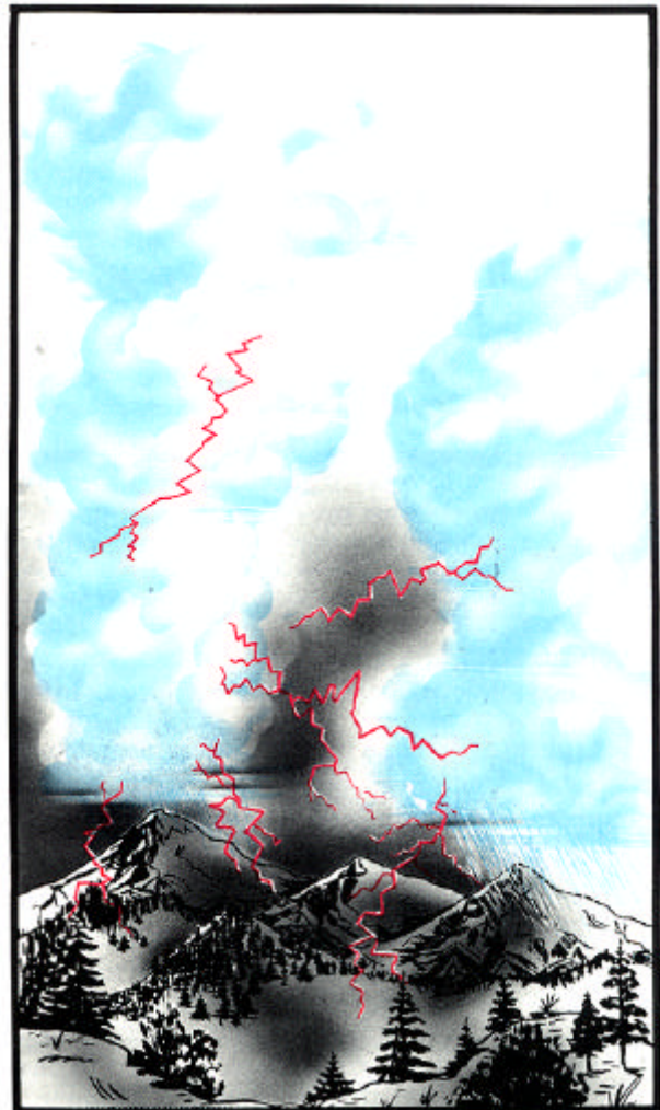
Lightning discharges take place within a cloud, from cloud-to-cloud, or from cloud-to-ground. Most discharges are within a cloud or from cloud-to-cloud, but the cloud-to-ground discharges are stronger. Lightning frequency is at a maximum in the mature stage.
